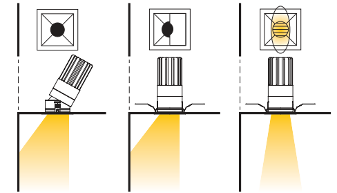
Adjustable Wall Wash Spreader Lens
